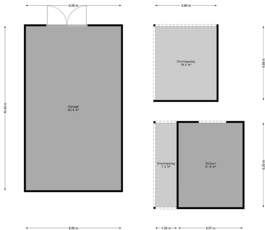
Garage
